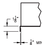
Flange Details
